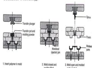
FIGURE 19.20 Sequence of operations in transfer molding for thermosetting plastics. This process is suitable particularly for intricate parts with varying wall thickness.
